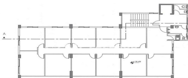
NEW FOURTH FLOOR SCALE 1:100
