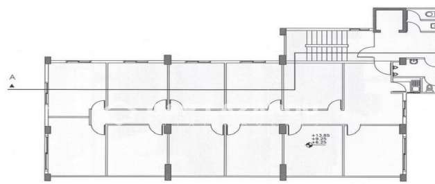
1st - 2nd - 3rd FLOOR EXISTING 1668/18.8.95 SCALE 1:100
