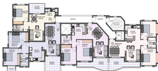
FIRST FLOOR PLAN BLOCK A
