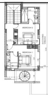
FIRST FLOOR
