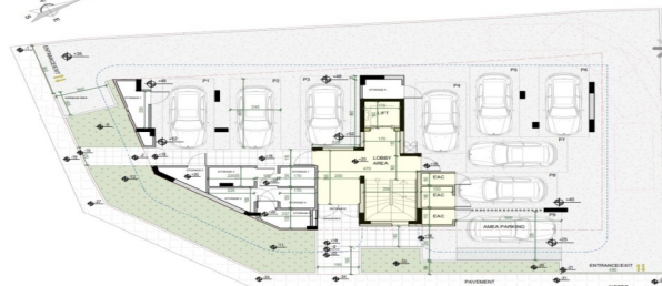
GROUND FLOOR PLAN SCALE 1:200
