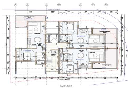
THIRD FLOOR
