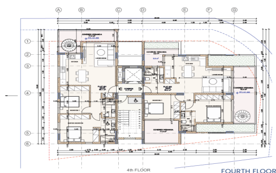
4th FLOOR
