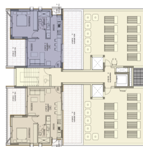
4th FLOOR
